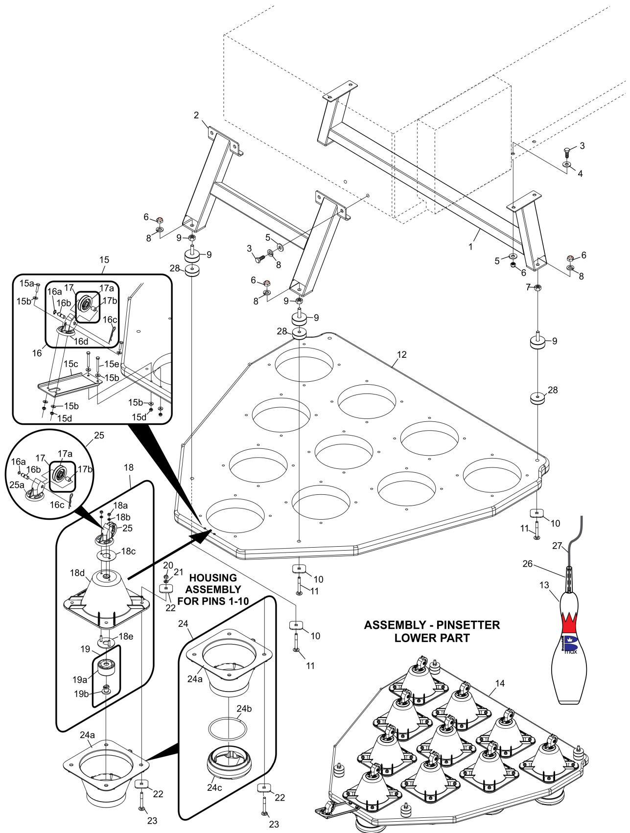
Boost Setting Platform Assembly (For Installations With Pin Bushings) - Ten Pin
